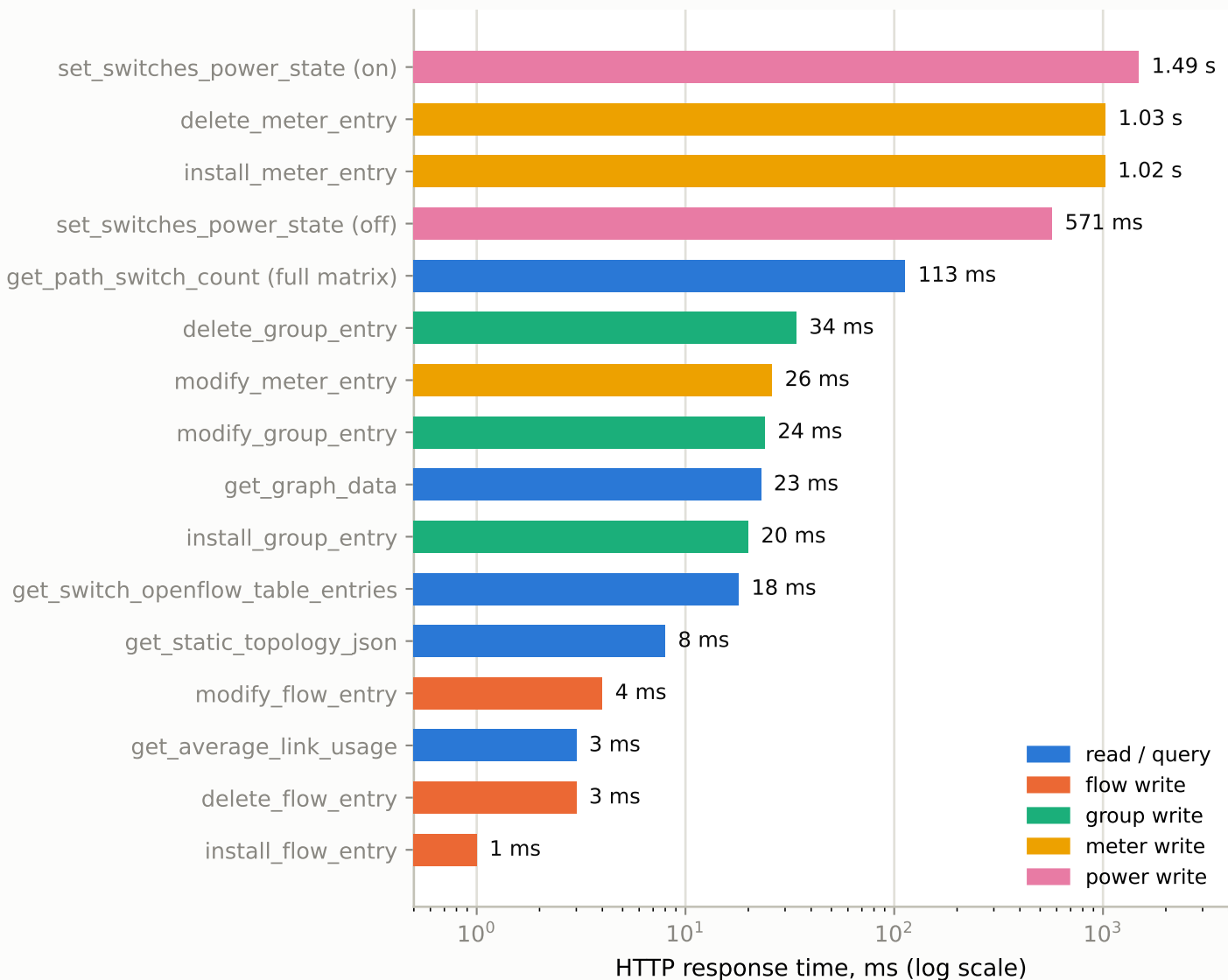
API response time by endpoint (OVS4, one sweep)
